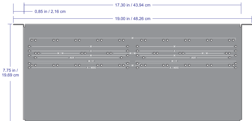
Mounting shelf – Underside
